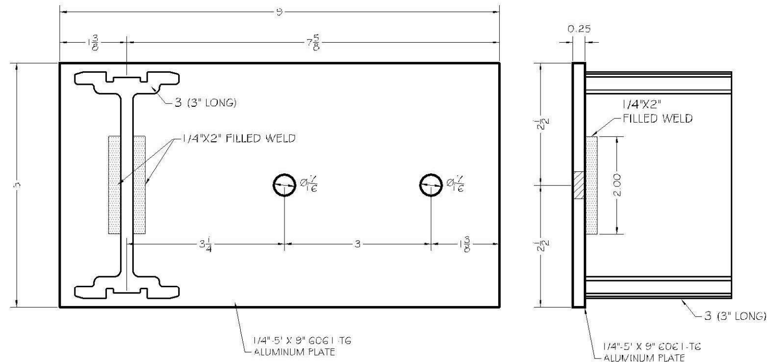
#27 - PGC-102 - "F" ANCHOR BRACKET
