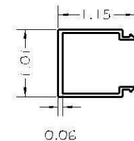
11- PGC-610 IG EXTERIOR FILLER COVER ALUMINUM ALLOY 6063-T6
