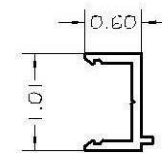
12- PGC-611 EXTERIOR FILLER BASE ALUMINUM ALLOY 6063-T6
