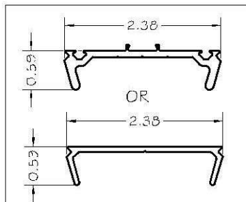
14- PGC-289 SNAP PLATE - ALUMINUM ALLOY 6063-T5
