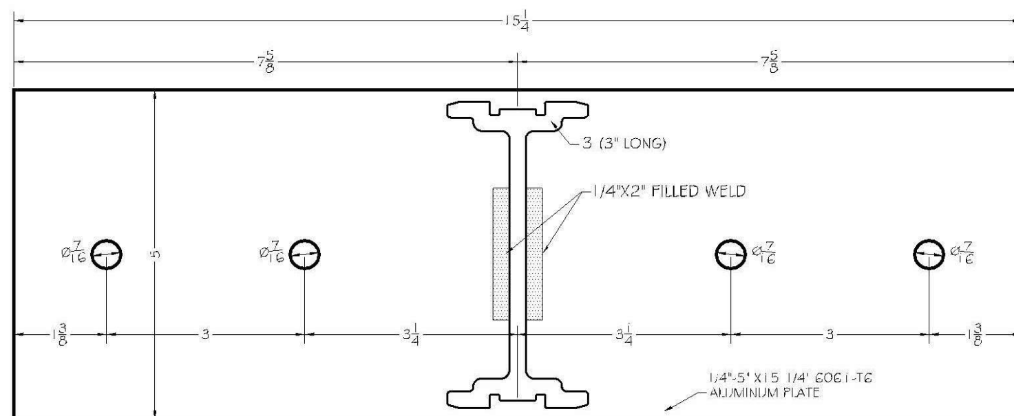
#28 - PGC-103 - "T" ANCHOR BRACKET
