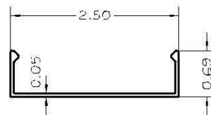
15- BPGC-2564 FACE COVER - ALUMINUM ALLOY 6063-T5
