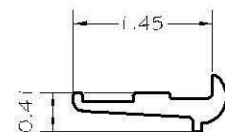
10- PGC-609, PGC-100 3" LONG SETTING CHAIR ALUMINUM ALLOY 6063-T6
