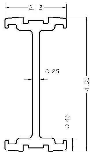
3- PGC-602 REINFORCEMENT SPLICE ALUMINUM ALLOY 6005-T5
