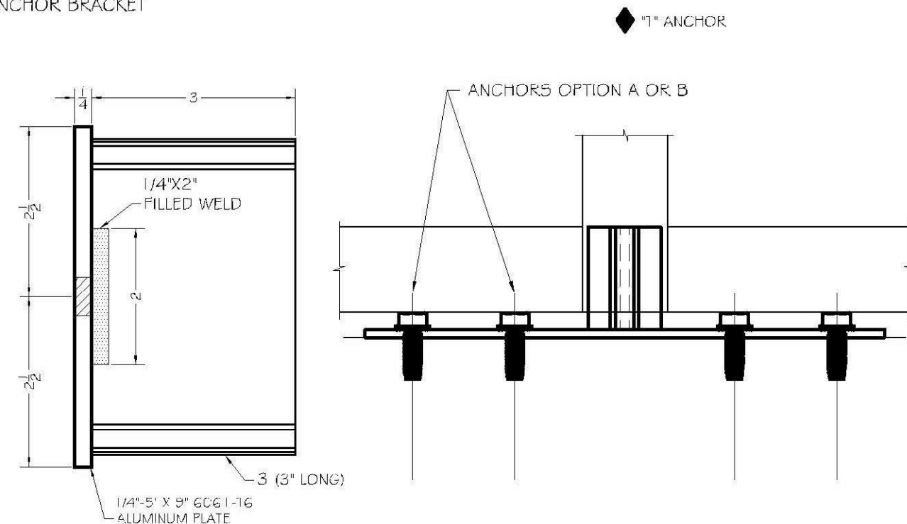
#28 - PGC-103 - "T" ANCHOR BRACKET
