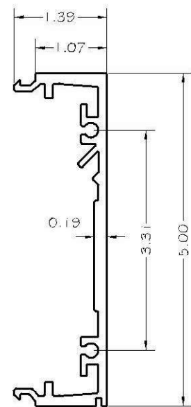
1- PGC-600 SSG MALE VERTICAL MULLION ALUMINUM ALLOY 6063-T6
