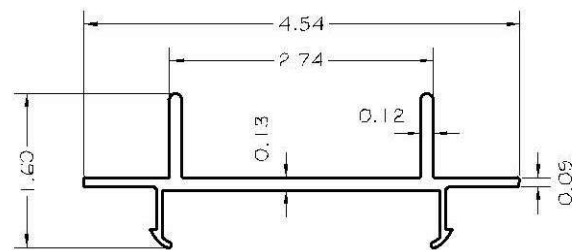
8- PGC-607 TOP RAIL ADAPTOR ALUMINUM ALLOY 6063-T6
