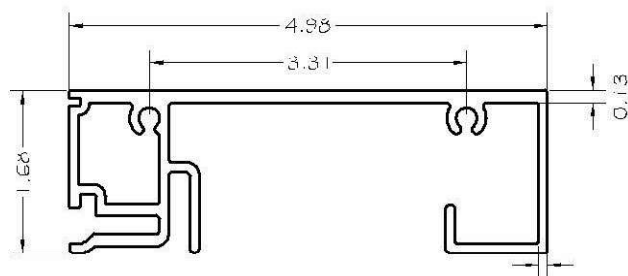
7- PGC-606 EXPANSION BOTTOM RAIL ALUMINUM ALLOY 6063-T6
