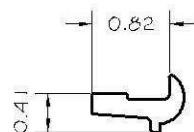
9- PGC-609, PGC-100 MODIFIED 3" LONG SETTING CHAIR ALUMINUM ALLOY 6063-T6
