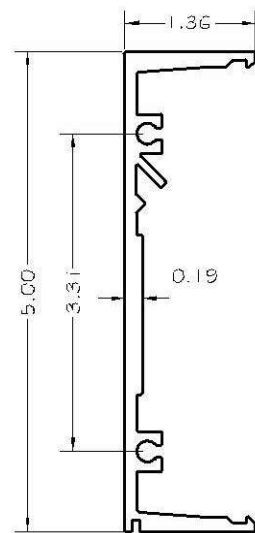
2- PGC-601 SSG FEMALE VERTICAL MULLION ALUMINUM ALLOY 6063-T6
