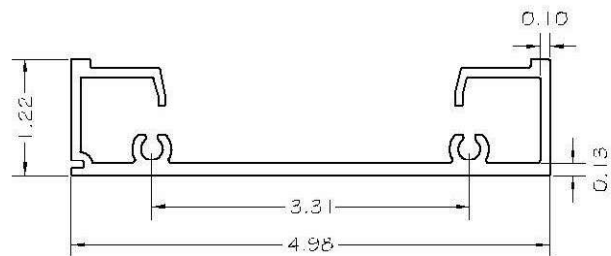
6- PGC-605 TOP RAIL ALUMINUM ALLOY 6063-T6
